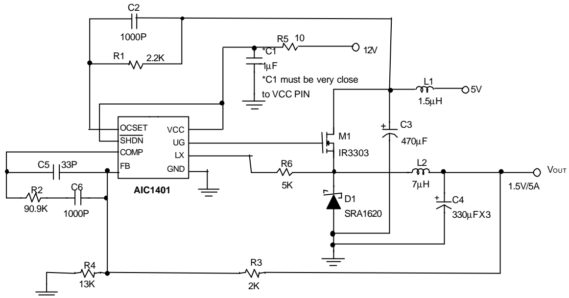
DC/DC Converter
