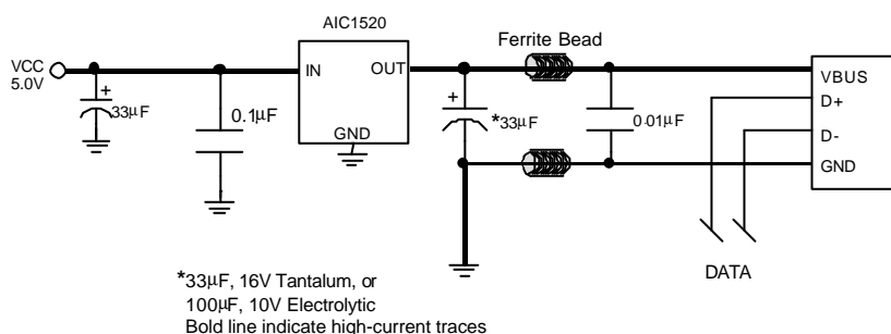
USB High-Side Power Switch
