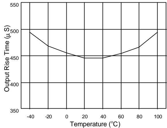
Fig. 8 Output Rise Time vs. temperature
