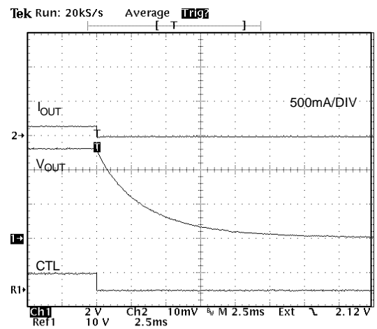
Fig. 15 Turn Off Falling Time (35Ω, 100μF Loading)
