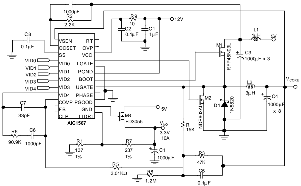
Switching DC/DC Converter
