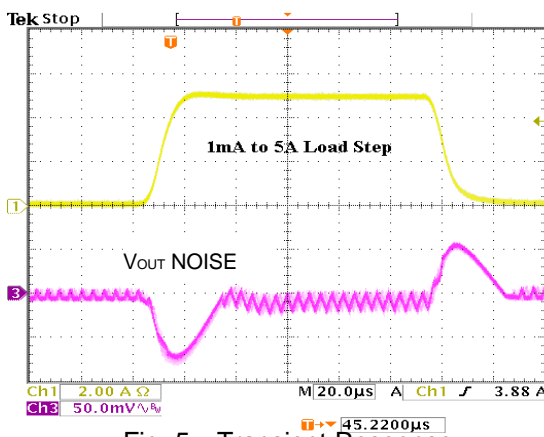
Fig. 5 Transient Response
