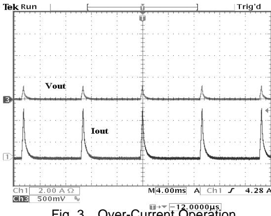
Fig. 3 Over-Current Operation
