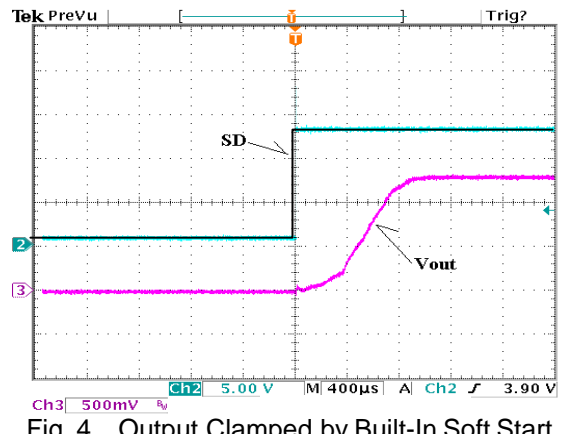
Fig. 4 Output Clamped by Built-In Soft Start
