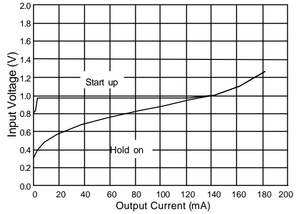
Fig. 10 AIC1641-30 Start-up & Hold-on Voltage (L=33µH)
