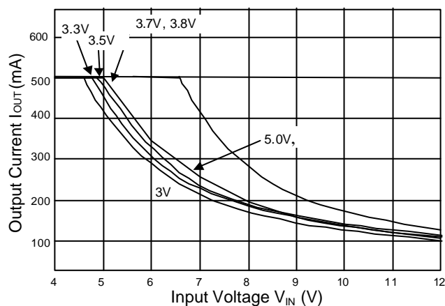
Fig. 2 Recommended Max. Output Current vs. Input Voltage
