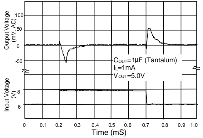
Fig. 4 Line Transient Response
