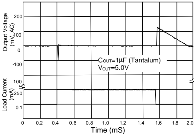
Fig. 5 Load Transient Response
