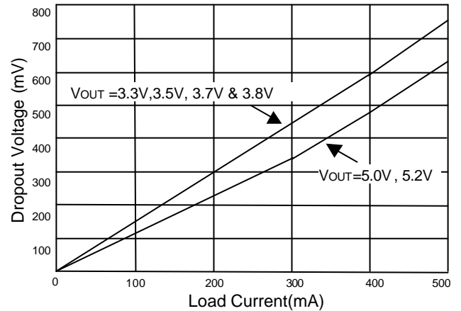
Fig. 6 Dropout Voltage vs. Load Current
