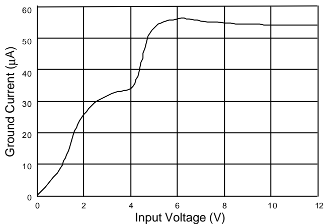
Fig. 1 Ground Current vs. Input Voltage
