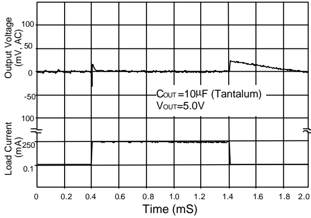
Fig. 3 Load Transient Response
