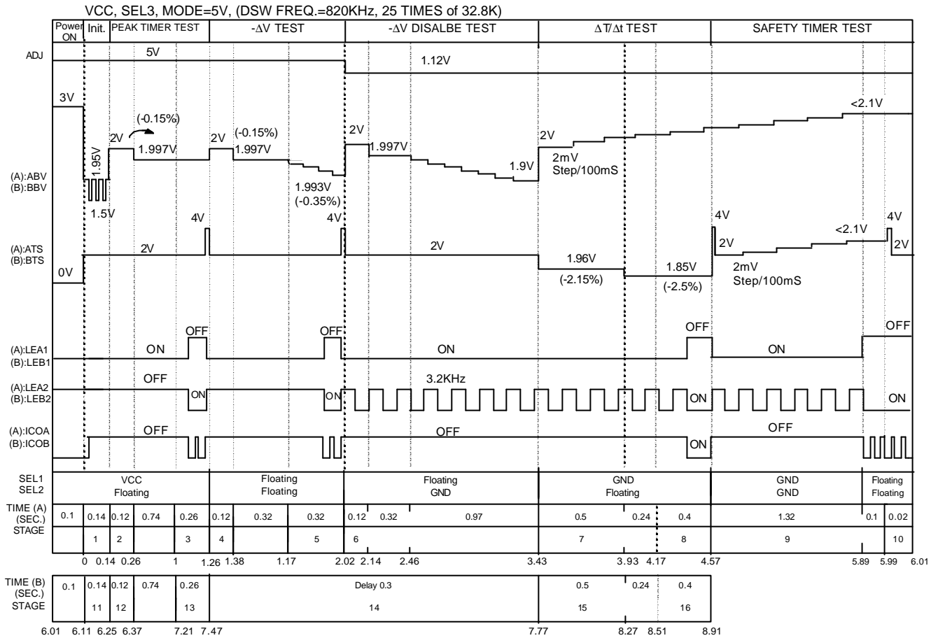
Fig. 17 Timing Diagram of AIC1782 in Test Mode
