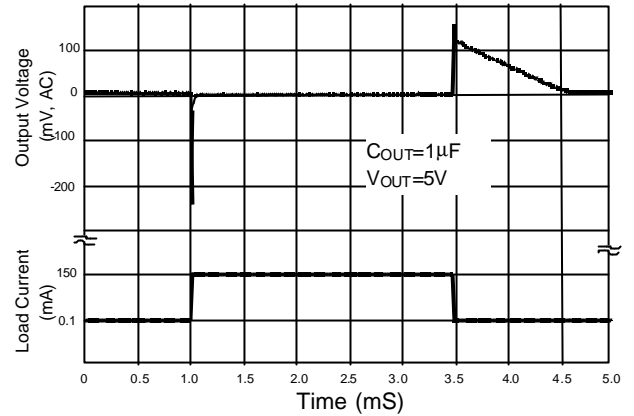
Fig. 8 Load Transient Response
