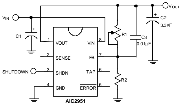
Fig. 13 Adjustable Regulator
