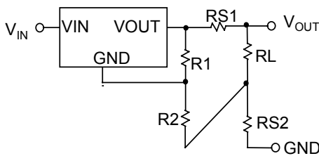
Figure 6 AIC LDO Adjustable regulator
