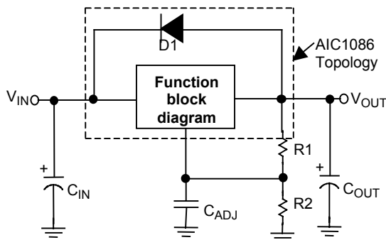
Figure 3 AIC1086 and bypass capacitor (C ADJ )
