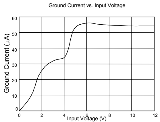
Figure 10 AIC1722 input and ground current characteristics
