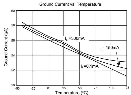
Figure 11 AIC 1722 temperature and ground current characteristics
