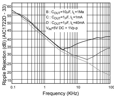
Figure 4 AIC 1722D-33 frequency and ripple rejection
