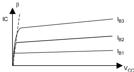
Figure 8 I-V characteristics of bipolar transistors
