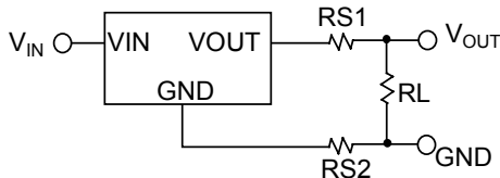
Figure 5 AIC LDO Fixed Regulator
