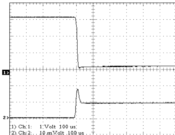
Figure 1 AIC1086 current limit test
