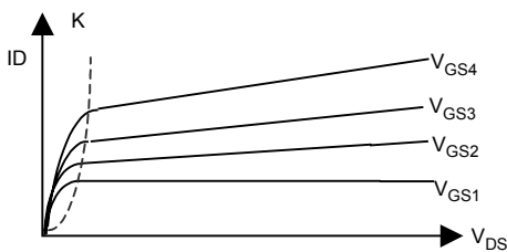
Figure 9 I-V characteristic of MOS transistors
