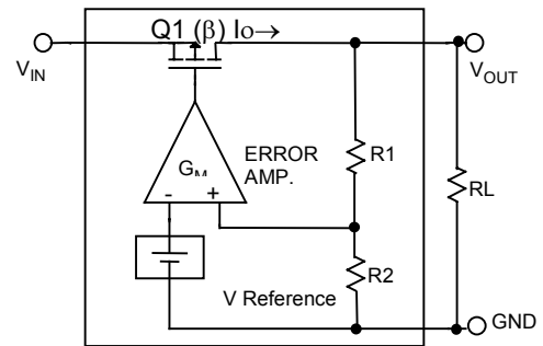
Figure 7 PMOS voltage regulator
