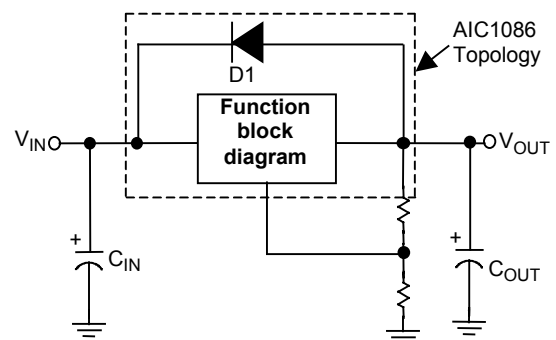
Figure 2 AIC1086 protection diodes diagram
