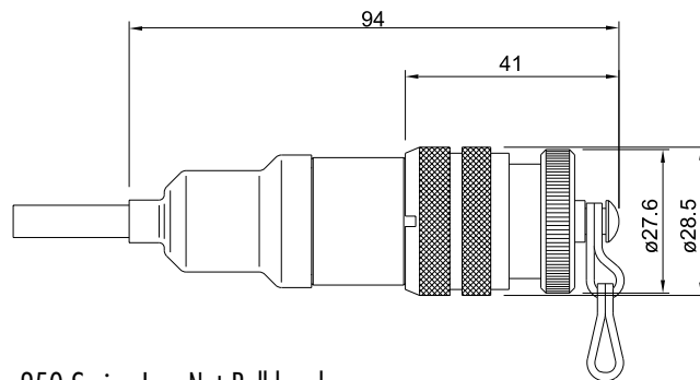
950 Series Jam Nut Bulkhead
