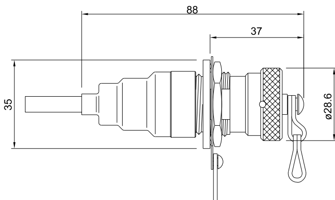
950 Series Jam Nut Bulkhead
