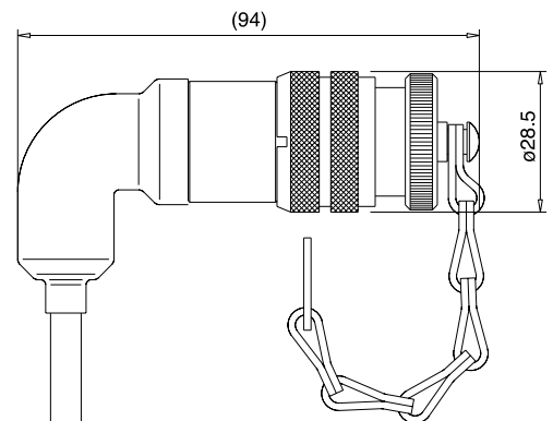
950 Series Right Angled Plug
